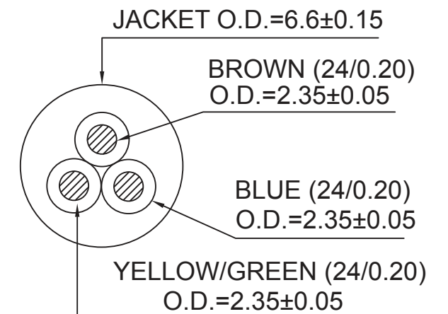
CROSS-SECTION VIEW
