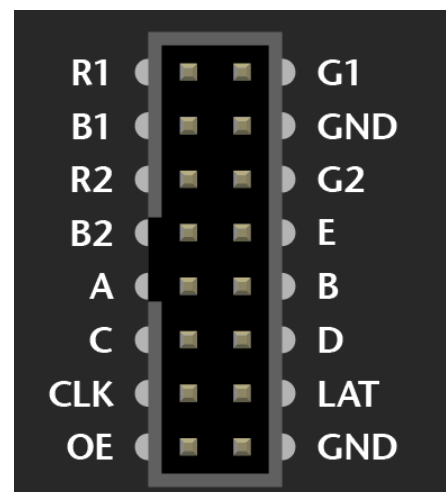
Pinout
