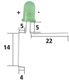
12 x LED6
