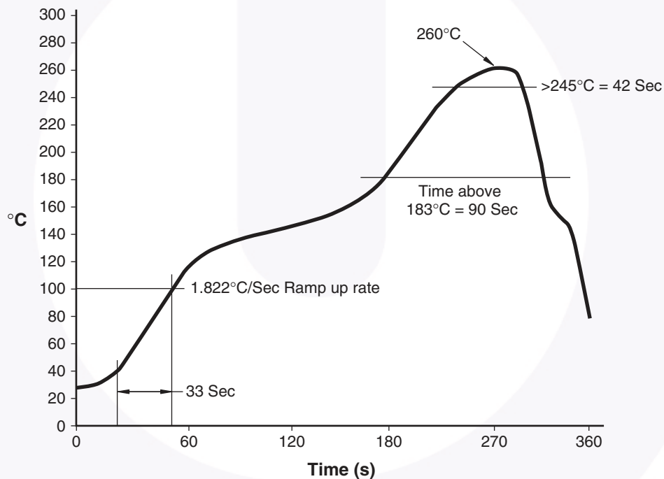
Figure 10. Reflow Profile
