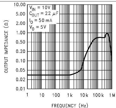
Figure 22. Output Impedance
